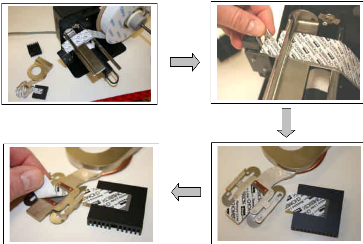
Figure 2 – Peel and Stick Application of T777 Material
